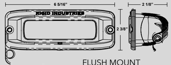
FLUSH MOUNT
